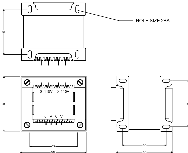
Outline Drawing Dual 115V Version
