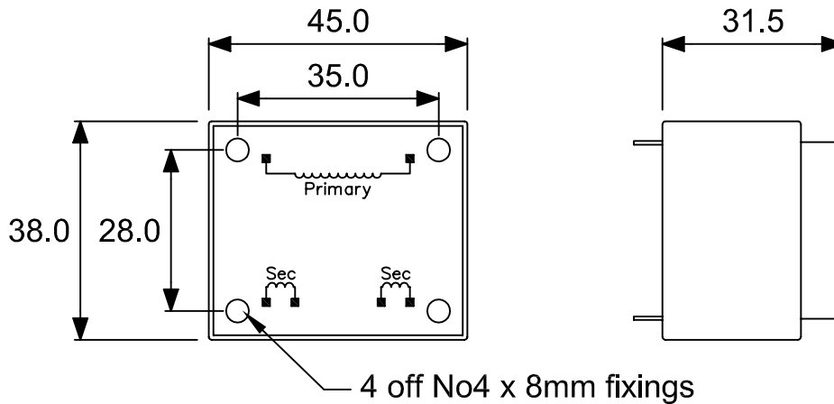
Outline Drawing
