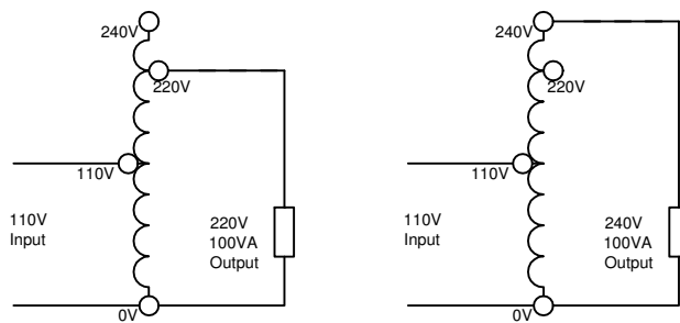
D3705 Connections
