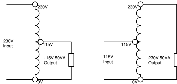
D3704 Connections
