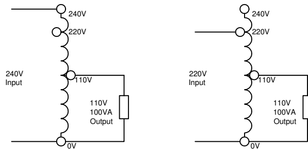
D3705 Connections
