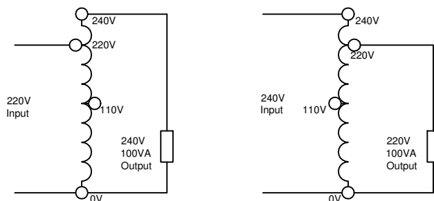
D3705 Connections
